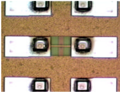
Fig. 2a. Shunt diode across 50 Ohm CPW lines
