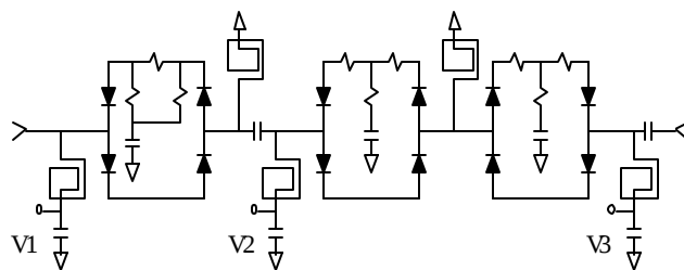
3 bit attenuator circuit schematic
