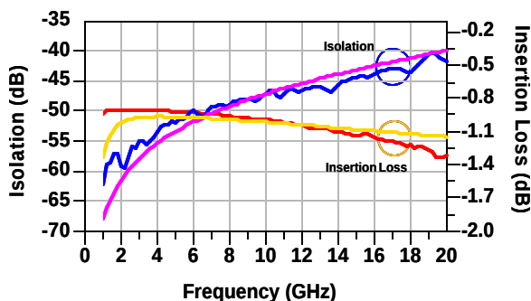
Fig. 3c. Measured and modeled switch performance
