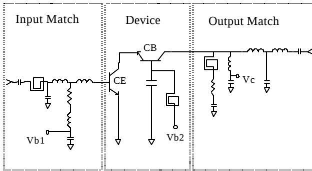
Fig. 15. Cascode amplifier circuit Schematic
