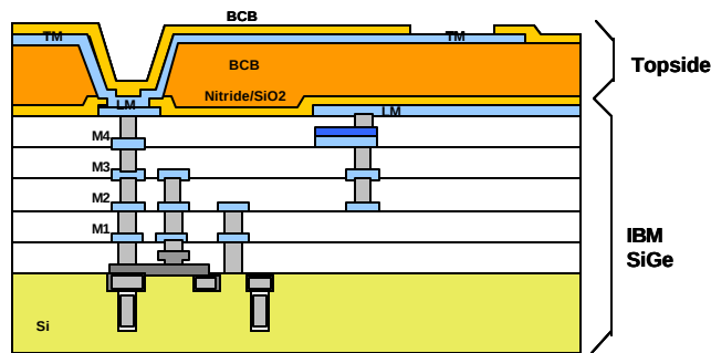
Fig.19. Cross-sectional view of the topside process
