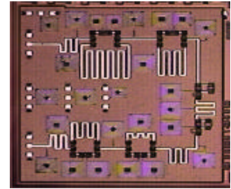
Fig. 8. 6-Bit Phase Shifter chip (3.8mm x 3.8mm)
