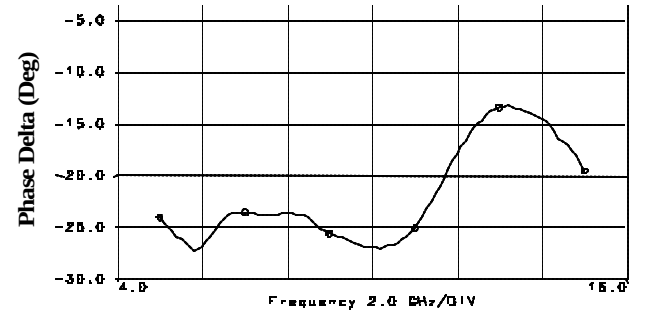
Fig. 18. Insertion phase delta between maximum and minimum gain states.
