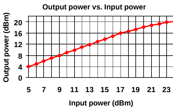
Fig. 3d. Switch input power 1-dB compression
