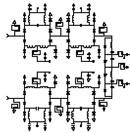
Fig. 8. 6-Bit Phase Shifter chip (3.8mm x 3.8mm)
