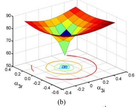
Fig.7 (a) ACPR@885kHz (dBc) and (b) 3 rd power correlation values (dB) vs. \tilde{a}_3
