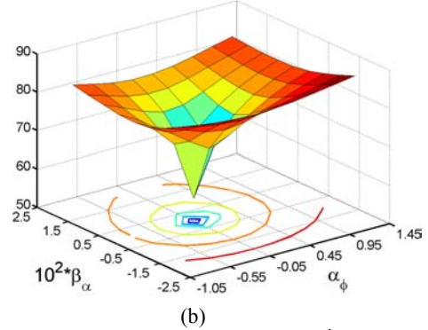
Fig.8 (a) ACPR@885kHz (dBc) and (b) 3 rd power correlation values (dB) vs. \beta_a and \alpha_\phi
