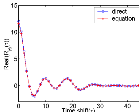
Fig.5 Output autocorrelation values of direct calculation (blue circles) and equation calculation (red stars)
