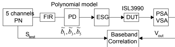
Fig.9 Measurement setup
