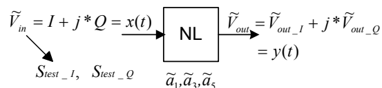
Fig.4 Complex polynomial input-output nonlinearity
